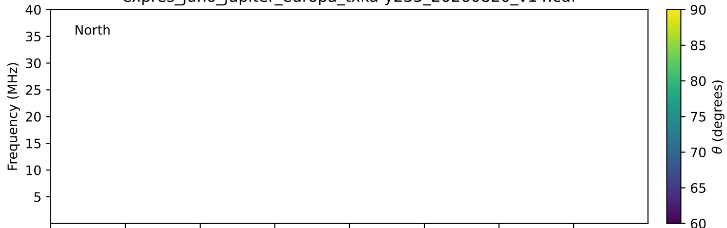
expres_juno_jupiter_europa_txka-y235_20260820_v14.cdf
