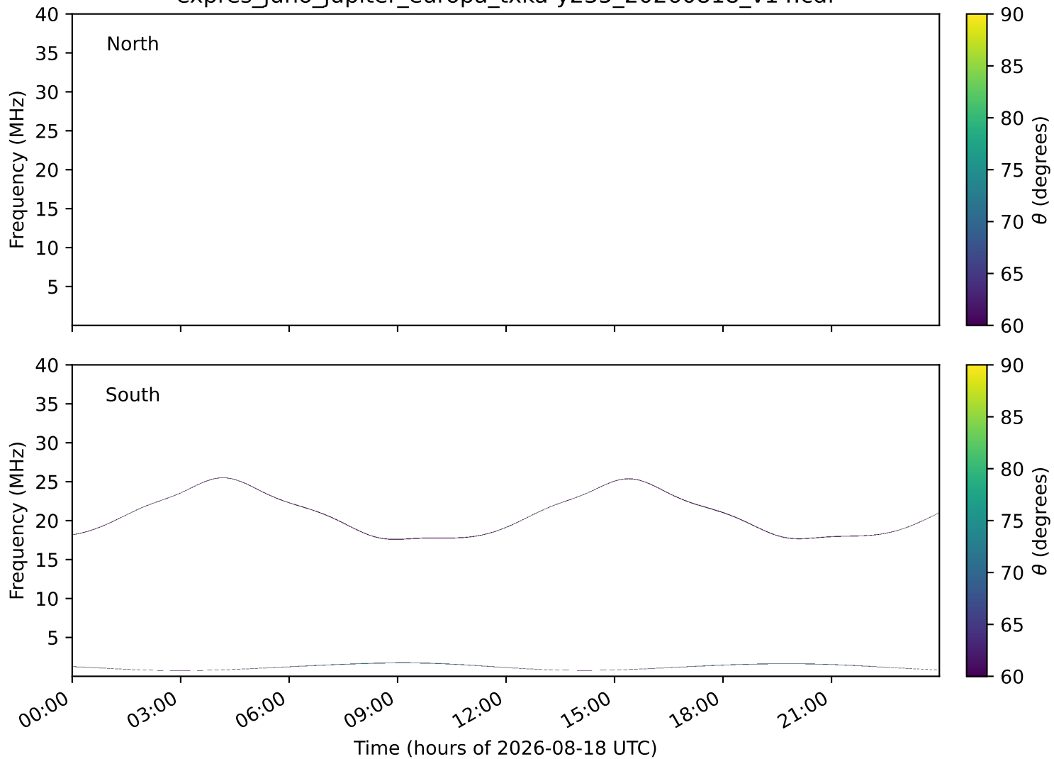
expres_juno_jupiter_europa_txka-y235_20260818_v14.cdf
