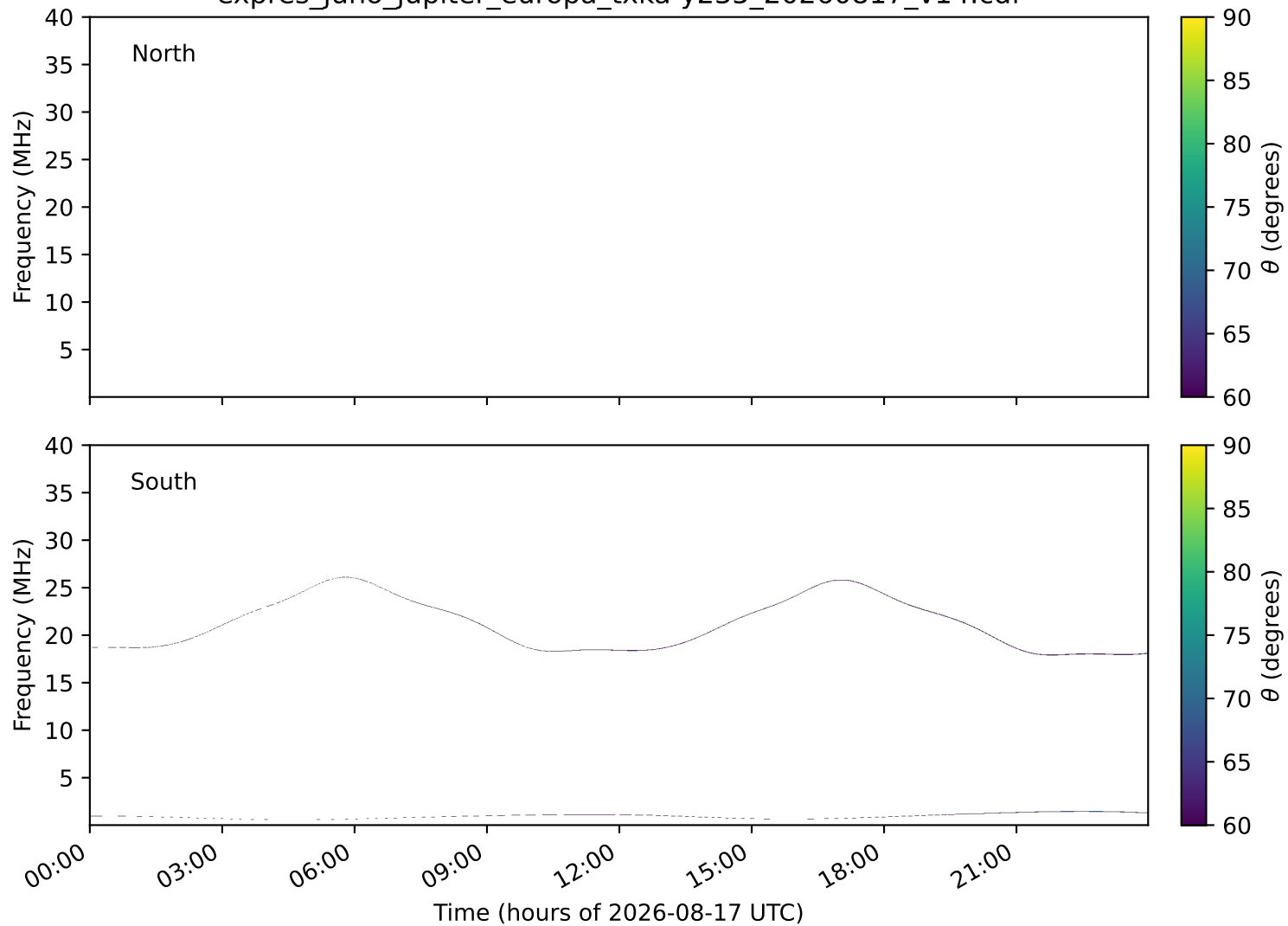
expres_juno_jupiter_europa_txka-y235_20260817_v14.cdf
