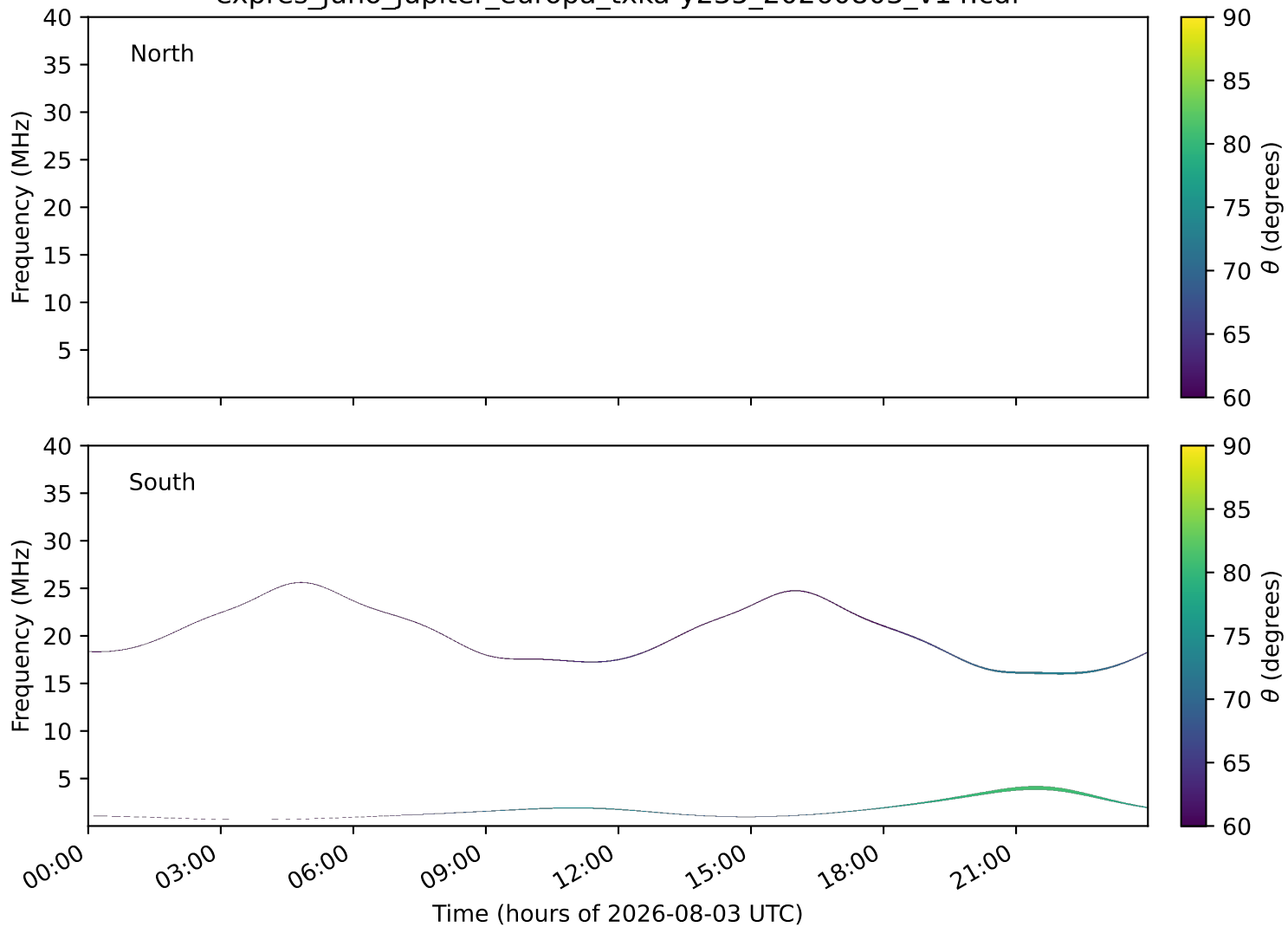
expres_juno_jupiter_europa_txka-y235_20260803_v14.cdf
