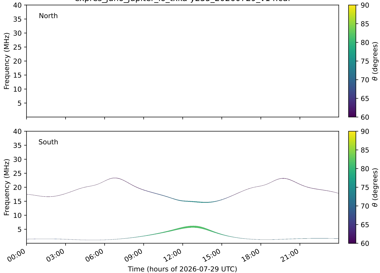
expres_juno_jupiter_io_txka-y235_20260729_v14.cdf
