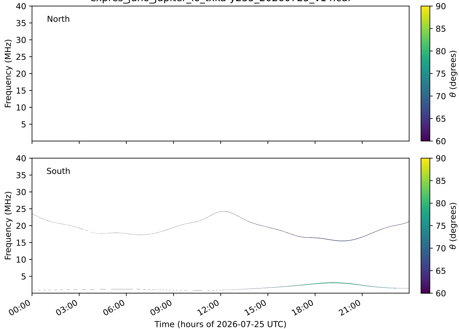
expres_juno_jupiter_io_txka-y235_20260725_v14.cdf
