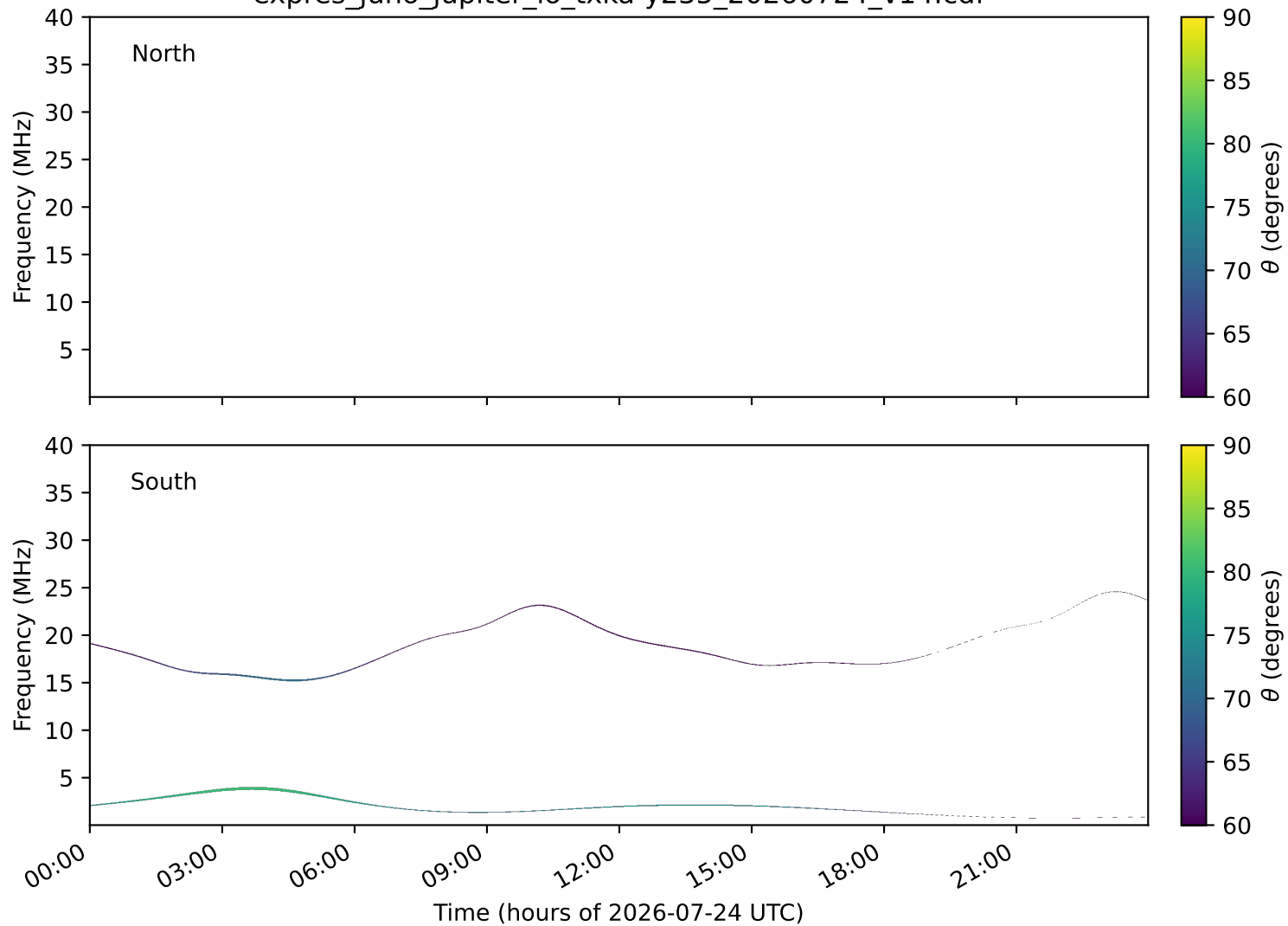
expres_juno_jupiter_io_txka-y235_20260724_v14.cdf
