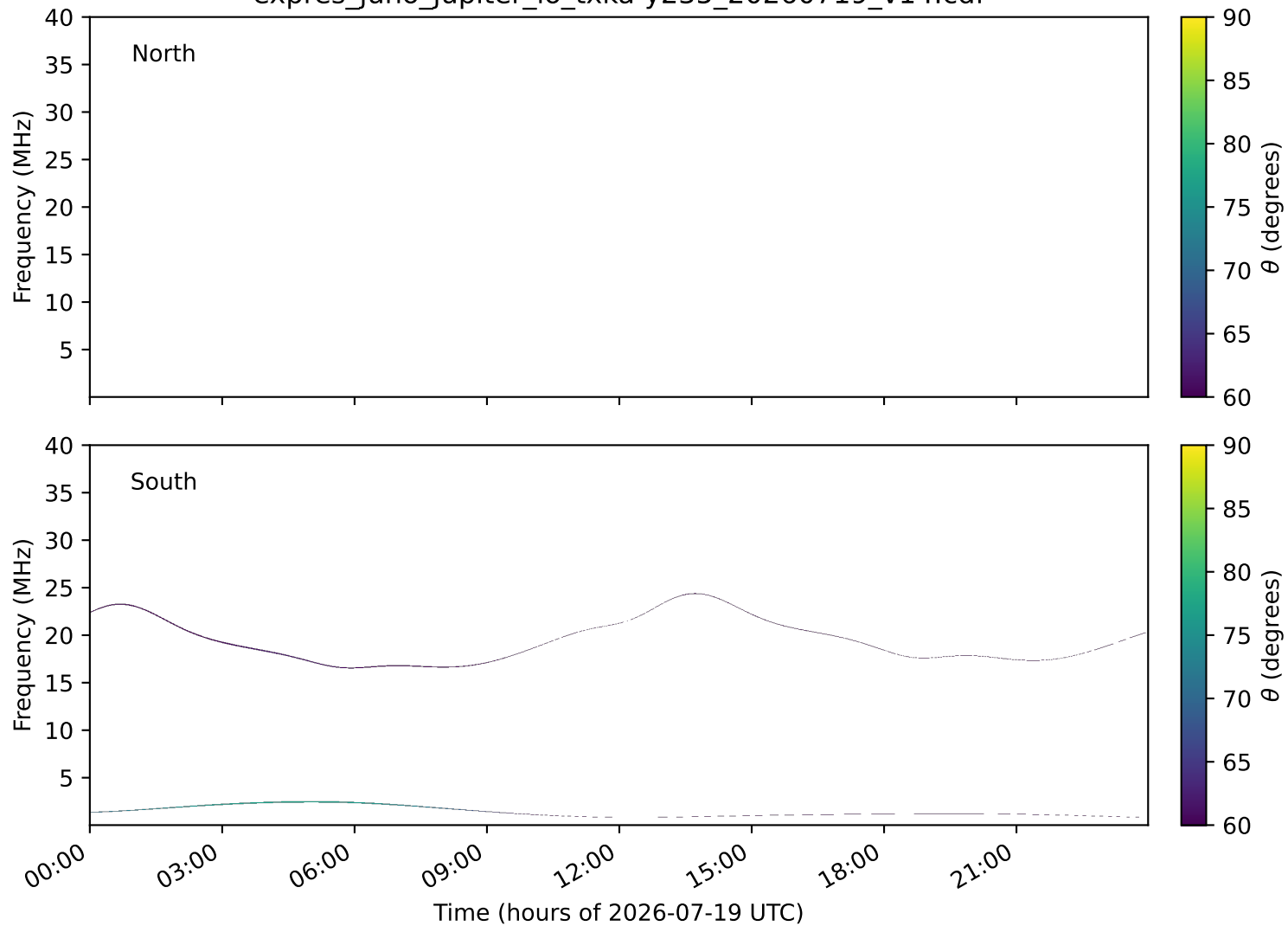
expres_juno_jupiter_io_txka-y235_20260719_v14.cdf
