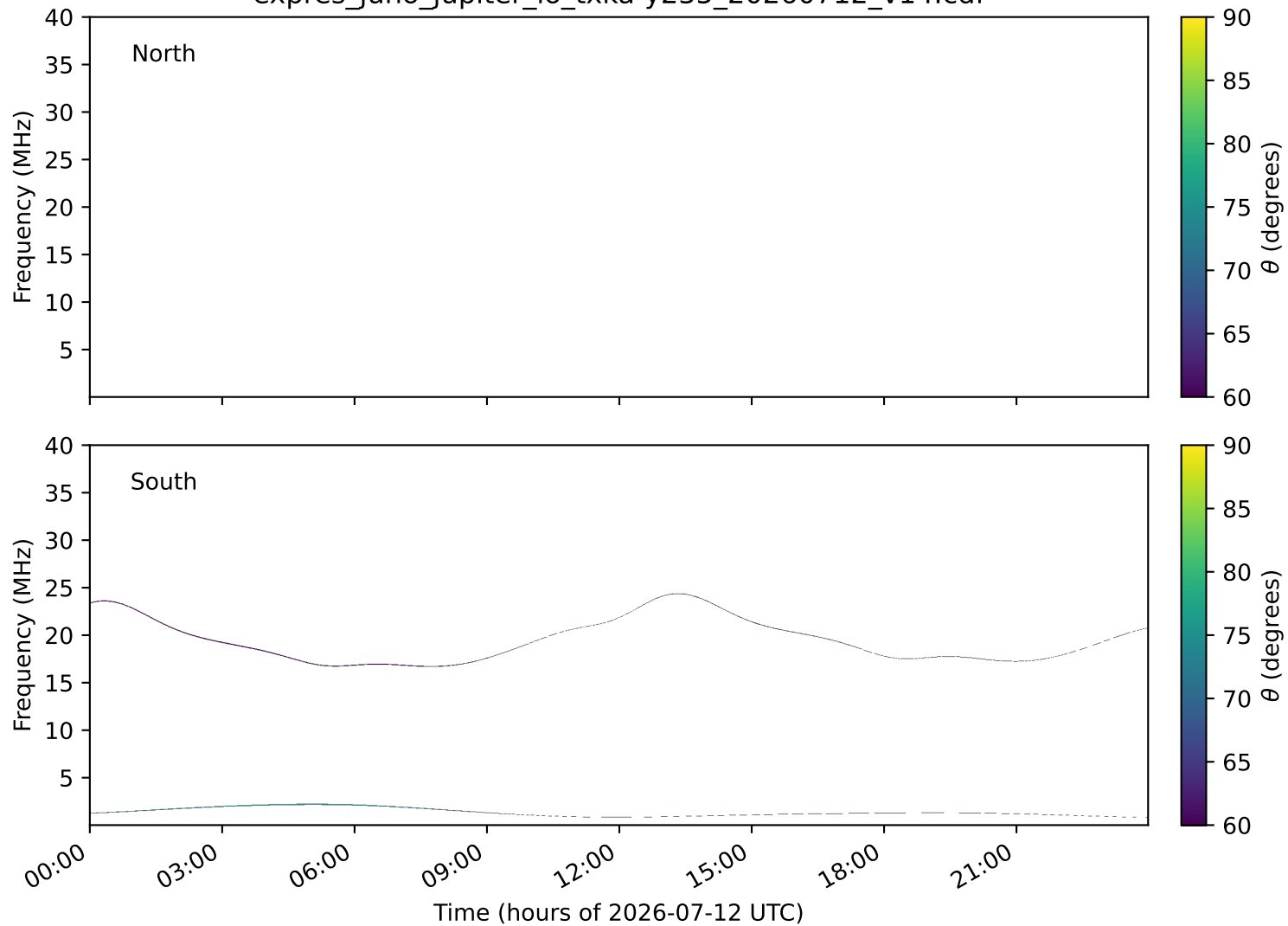
expres_juno_jupiter_io_txka-y235_20260712_v14.cdf
