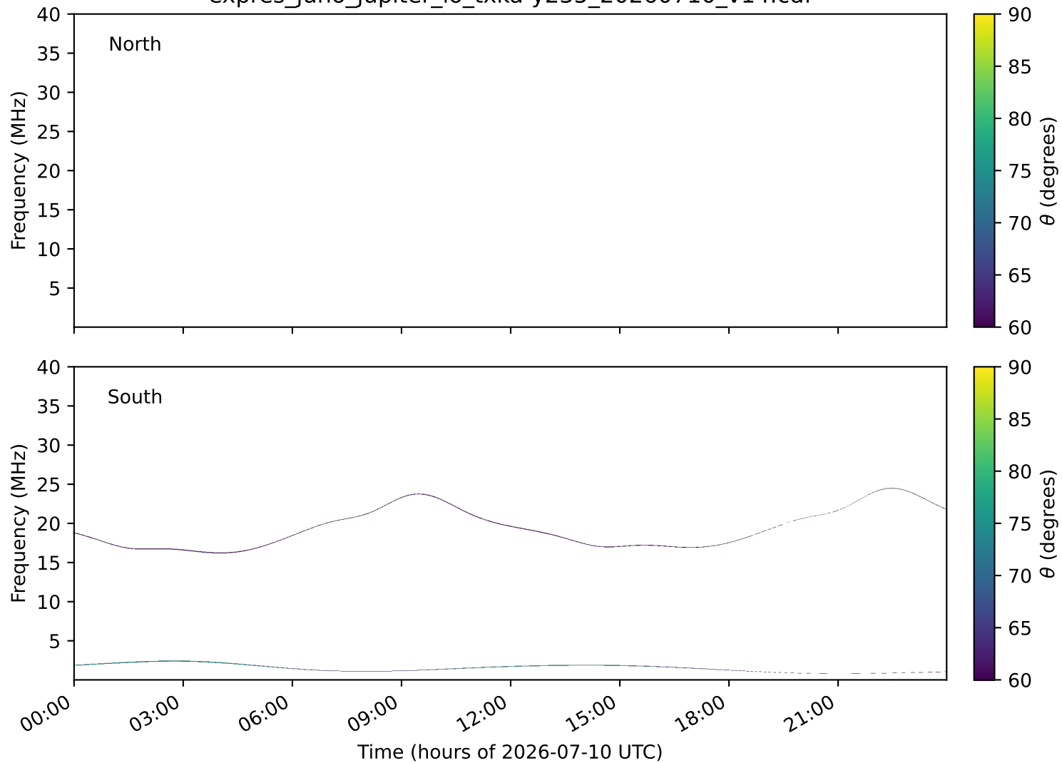
expres_juno_jupiter_io_txka-y235_20260710_v14.cdf
