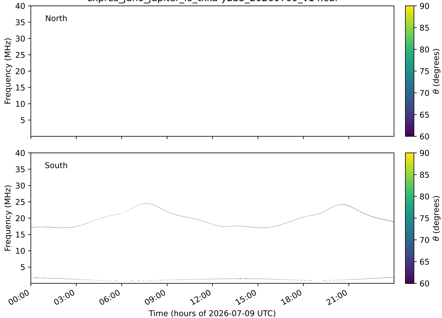
expres_juno_jupiter_io_txka-y235_20260709_v14.cdf
