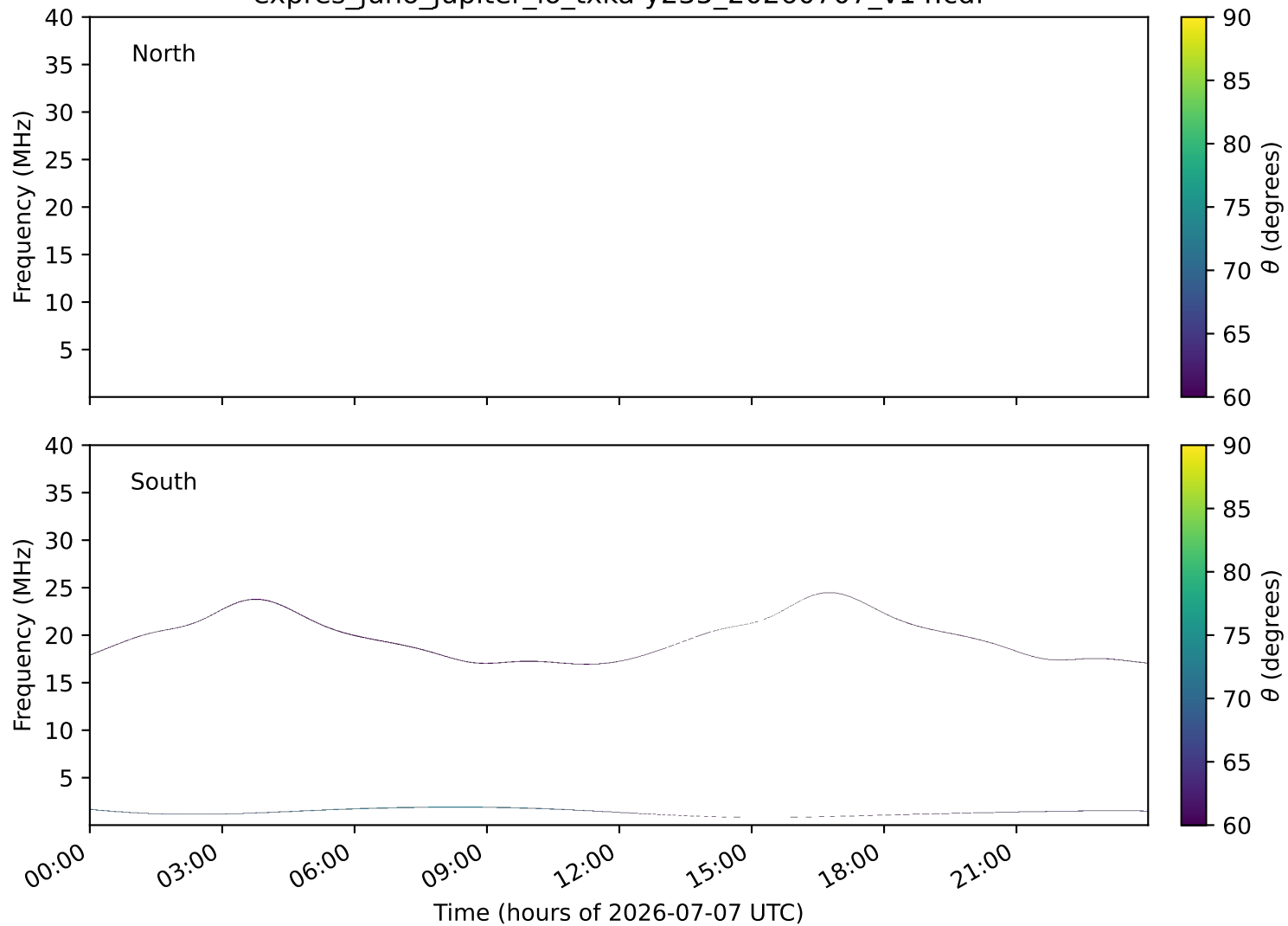
expres_juno_jupiter_io_txka-y235_20260707_v14.cdf
