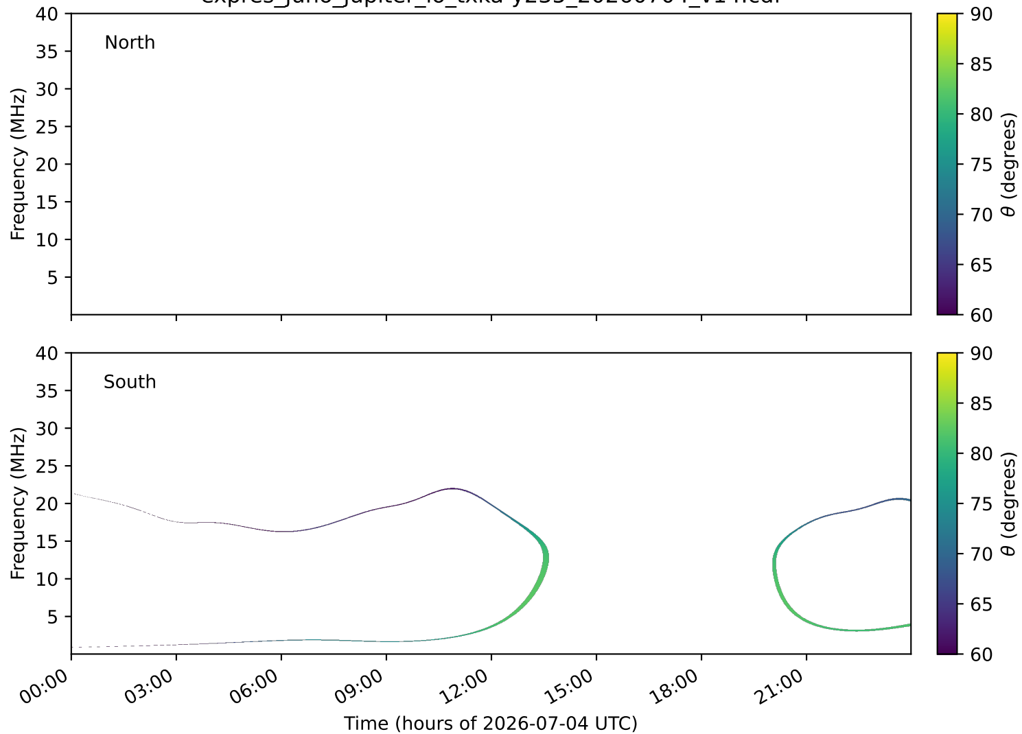
expres_juno_jupiter_io_txka-y235_20260704_v14.cdf
