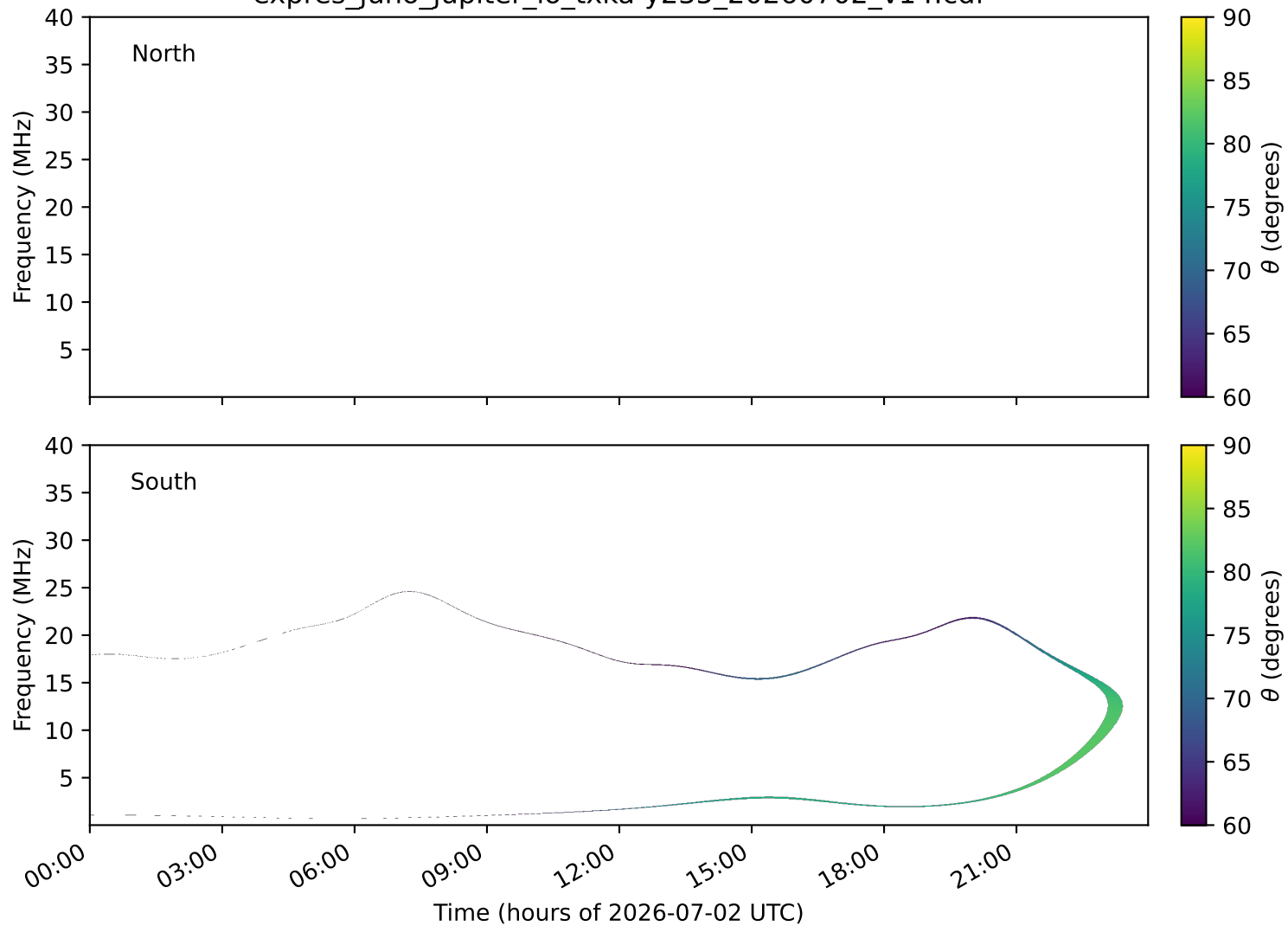
expres_juno_jupiter_io_txka-y235_20260702_v14.cdf
