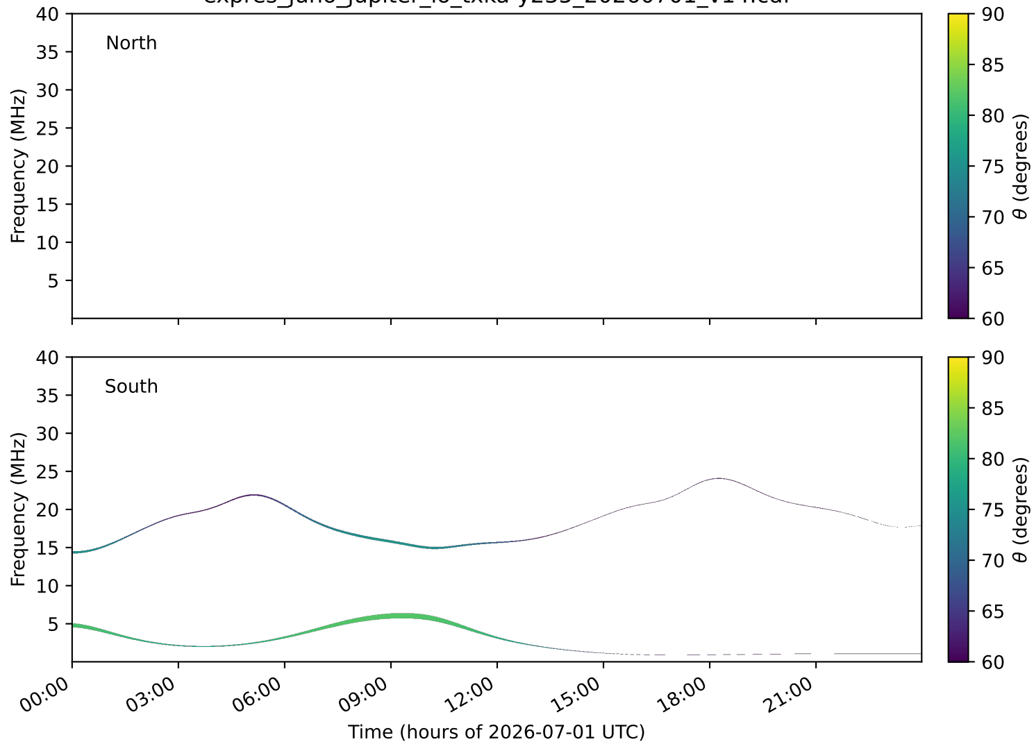
expres_juno_jupiter_io_txka-y235_20260701_v14.cdf
