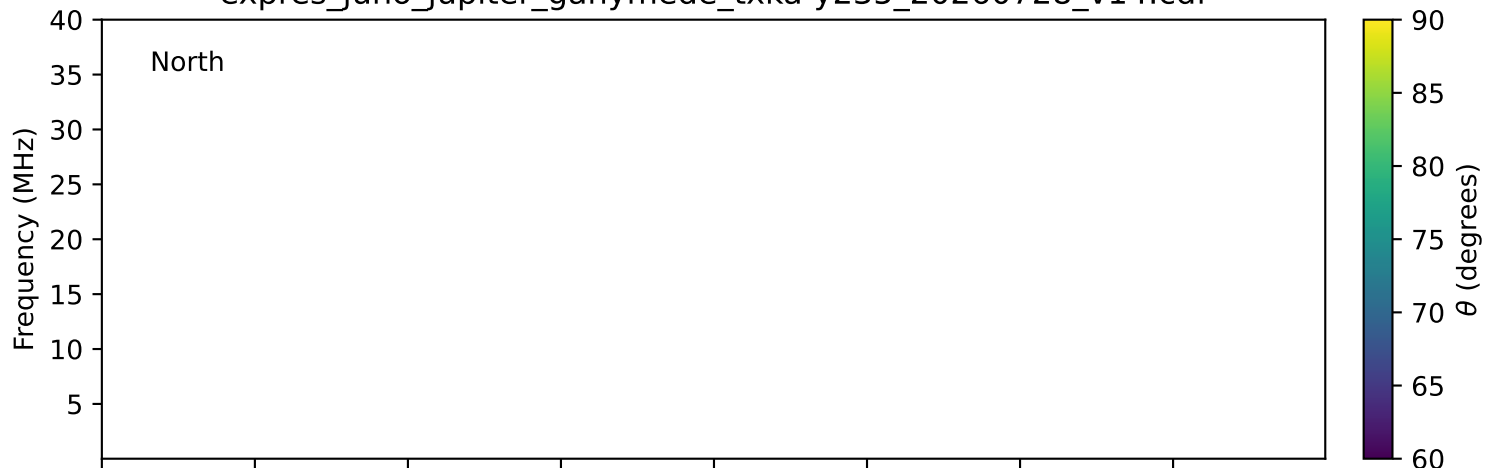
expres_juno_jupiter_ganymede_txka-y235_20260728_v14.cdf
