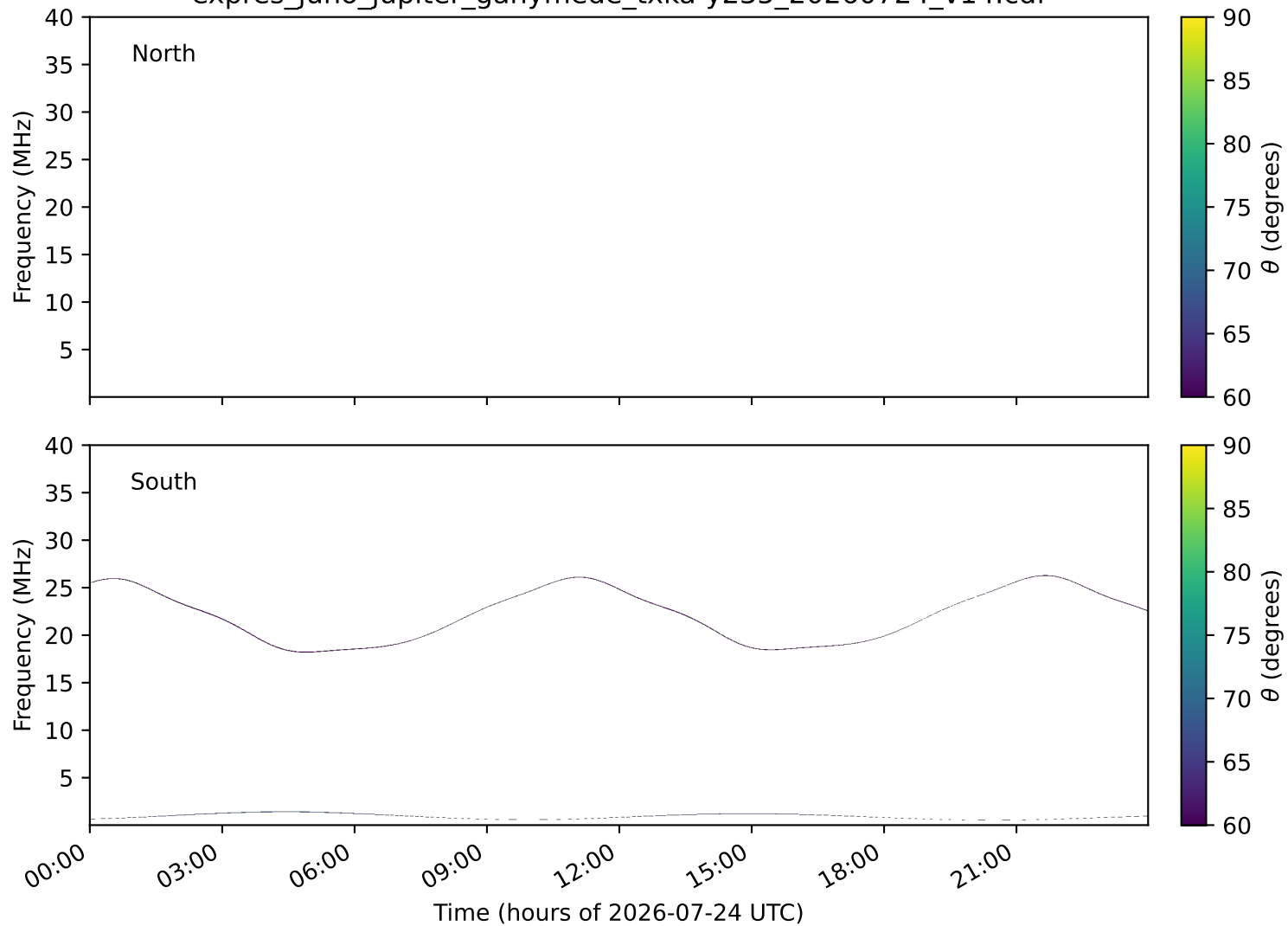
expres_juno_jupiter_ganymede_txka-y235_20260724_v14.cdf
