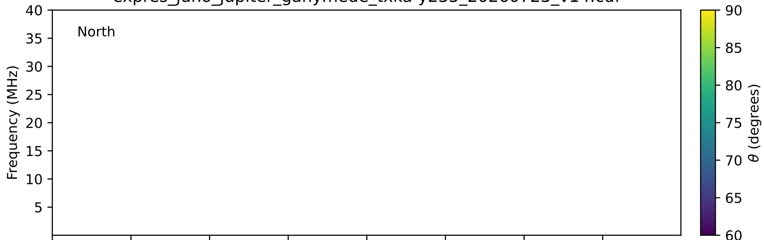
expres_juno_jupiter_ganymede_txka-y235_20260723_v14.cdf
