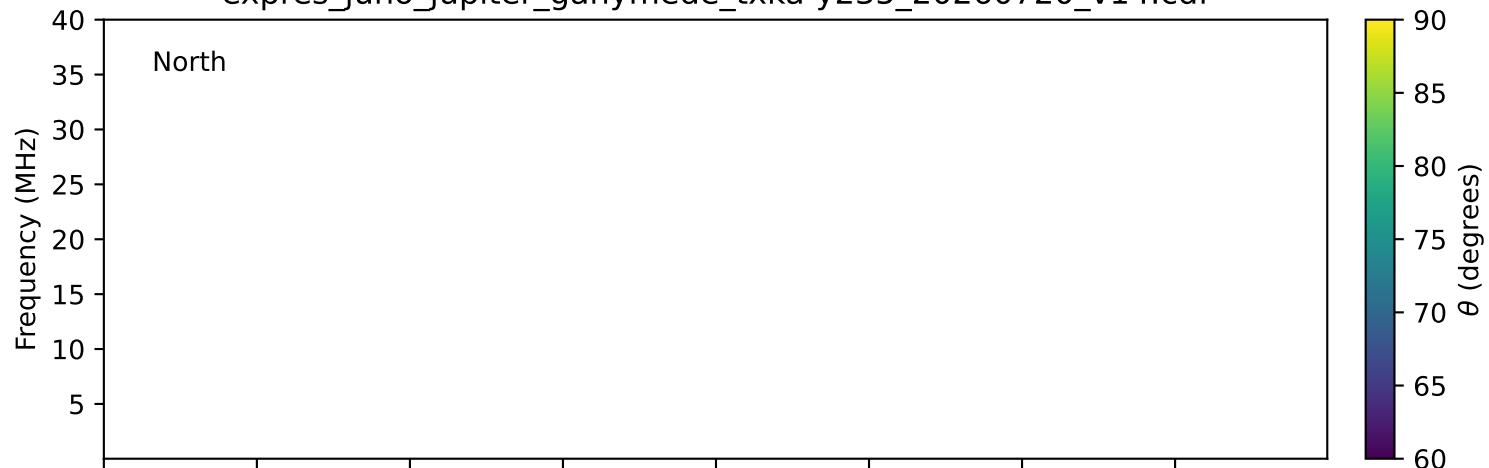
expres_juno_jupiter_ganymede_txka-y235_20260720_v14.cdf
