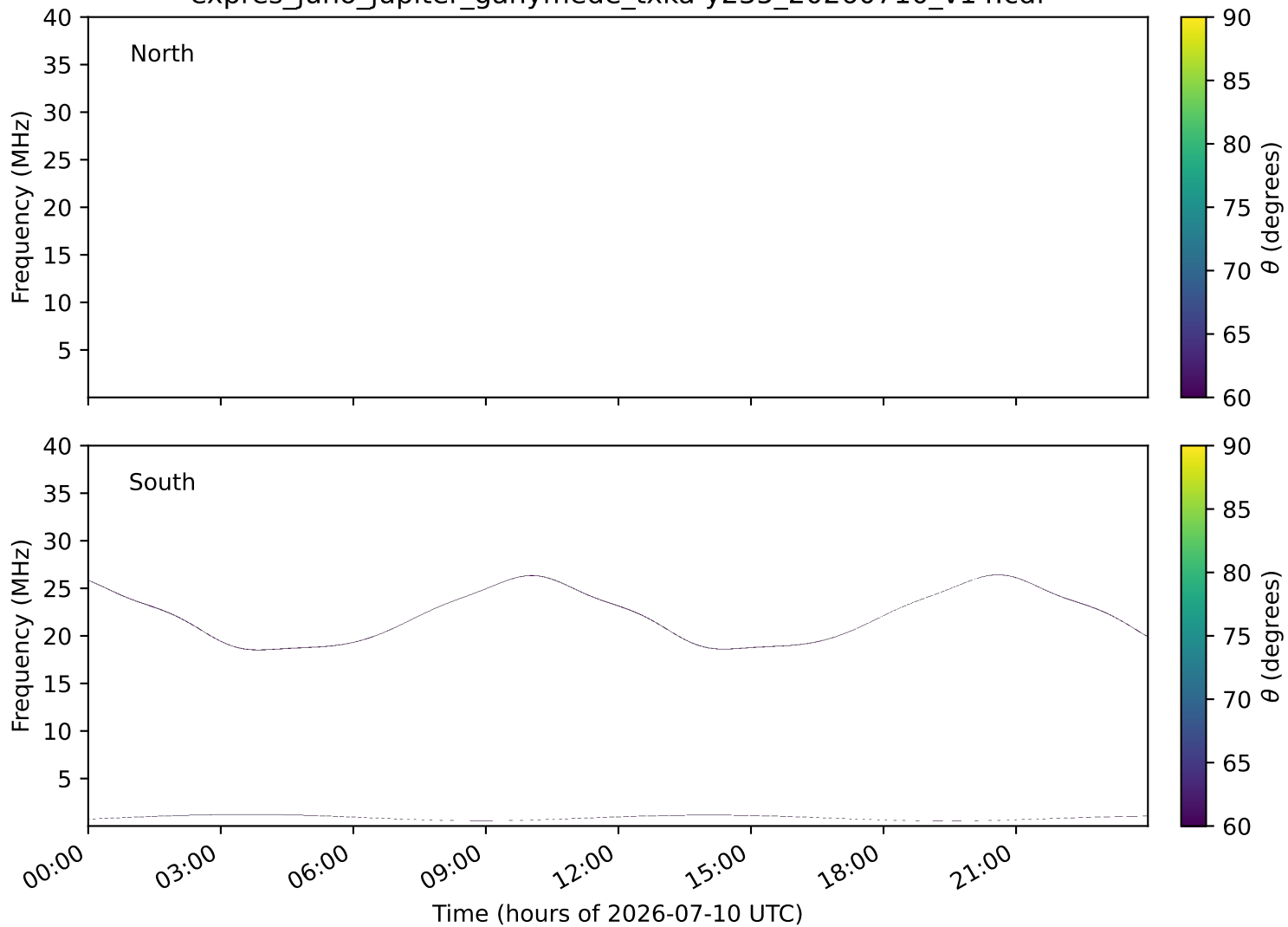
expres_juno_jupiter_ganymede_txka-y235_20260710_v14.cdf
