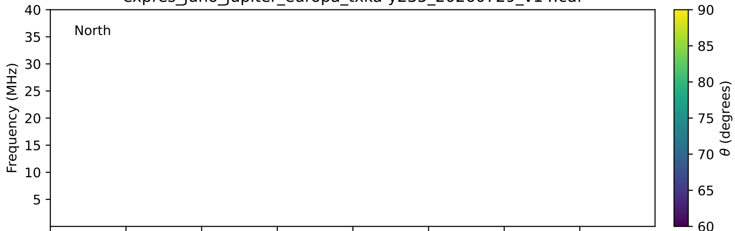
expres_juno_jupiter_europa_txka-y235_20260729_v14.cdf
