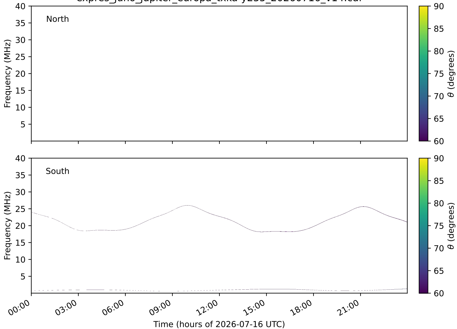
expres_juno_jupiter_europa_txka-y235_20260716_v14.cdf
