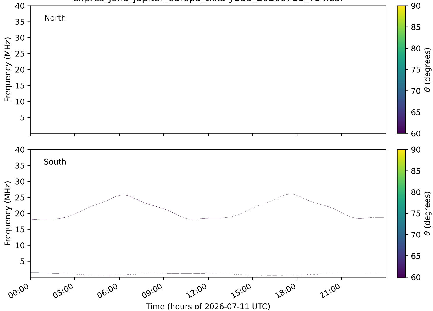
expres_juno_jupiter_europa_txka-y235_20260711_v14.cdf
