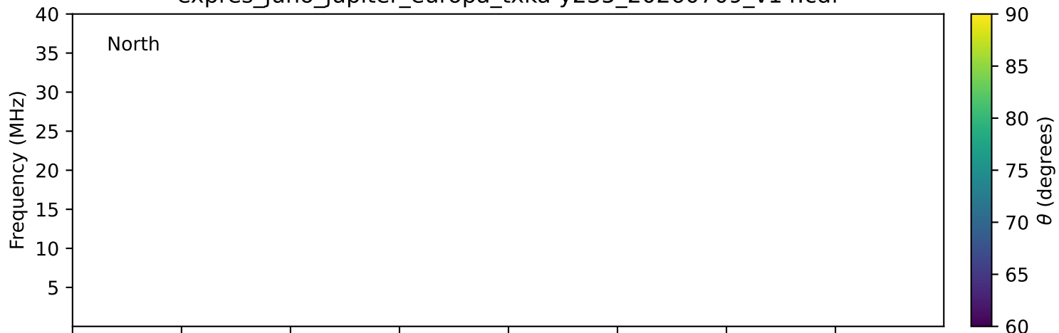
expres_juno_jupiter_europa_txka-y235_20260709_v14.cdf
