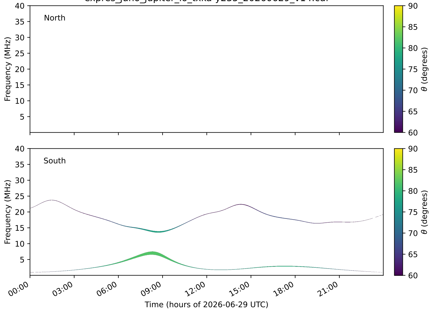
expres_juno_jupiter_io_txka-y235_20260629_v14.cdf
