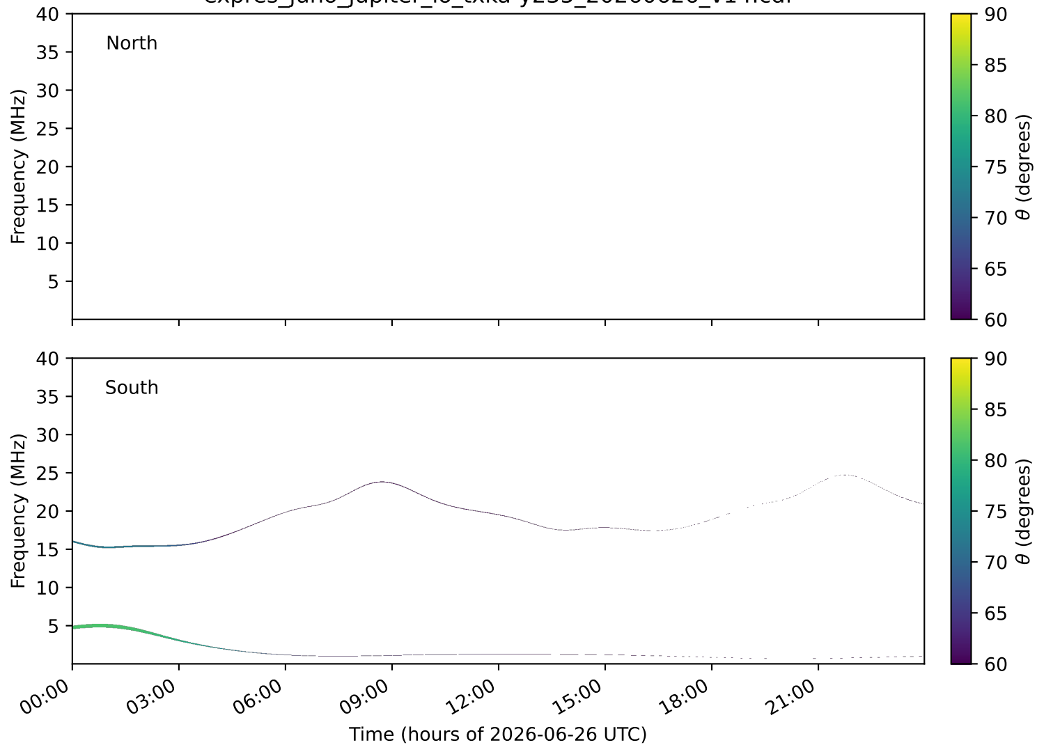
expres_juno_jupiter_io_txka-y235_20260626_v14.cdf
