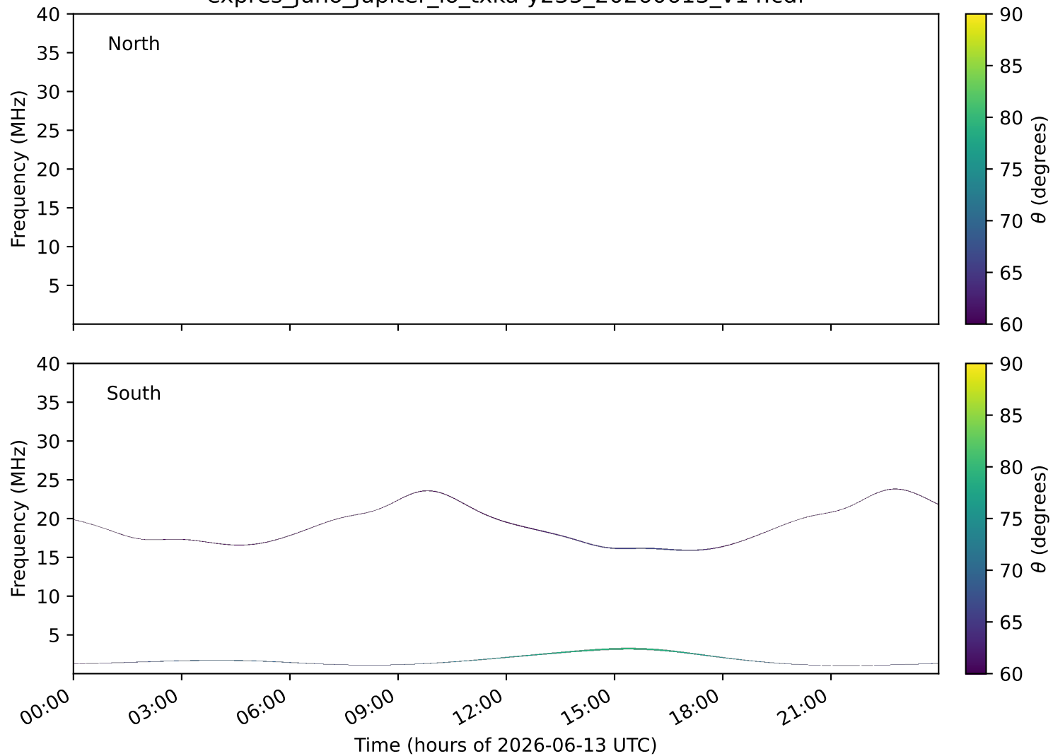
expres_juno_jupiter_io_txka-y235_20260613_v14.cdf
