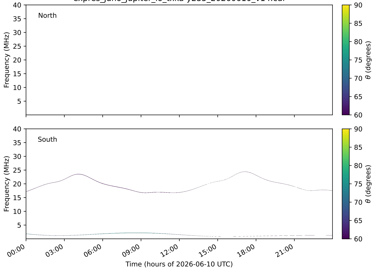
expres_juno_jupiter_io_txka-y235_20260610_v14.cdf
