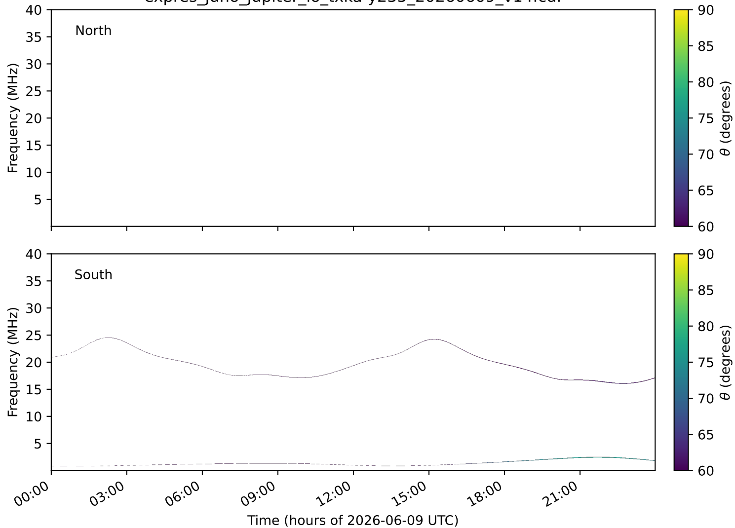
expres_juno_jupiter_io_txka-y235_20260609_v14.cdf
