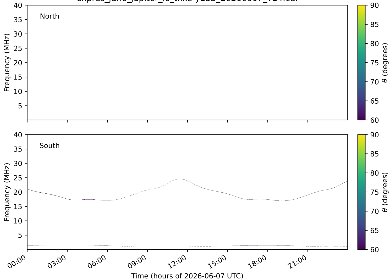
expres_juno_jupiter_io_txka-y235_20260607_v14.cdf
