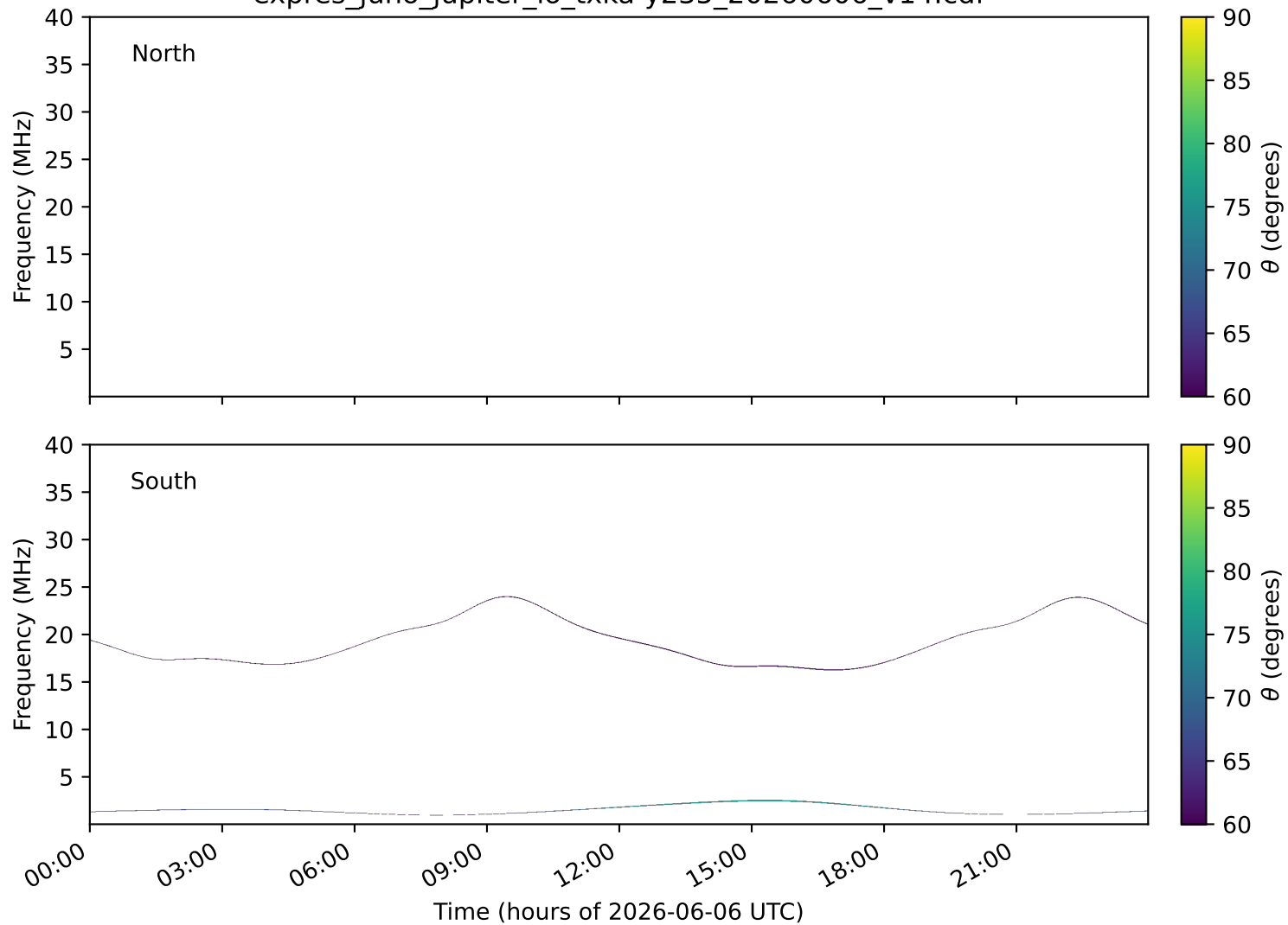
expres_juno_jupiter_io_txka-y235_20260606_v14.cdf
