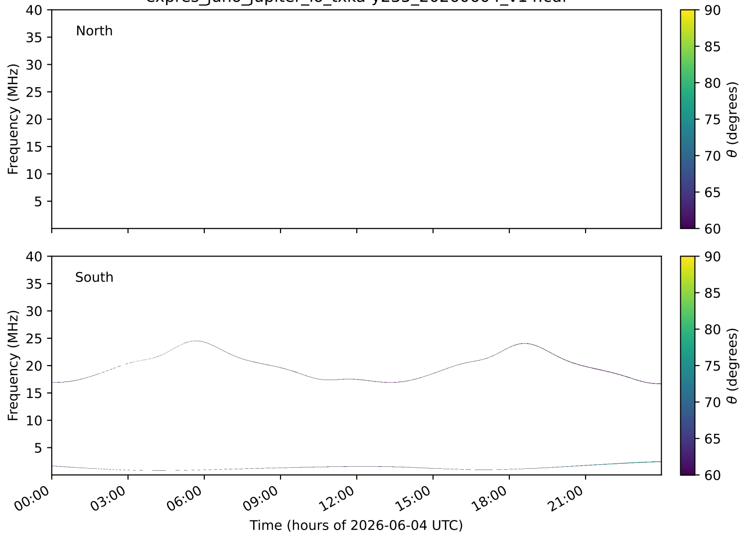
expres_juno_jupiter_io_txka-y235_20260604_v14.cdf
