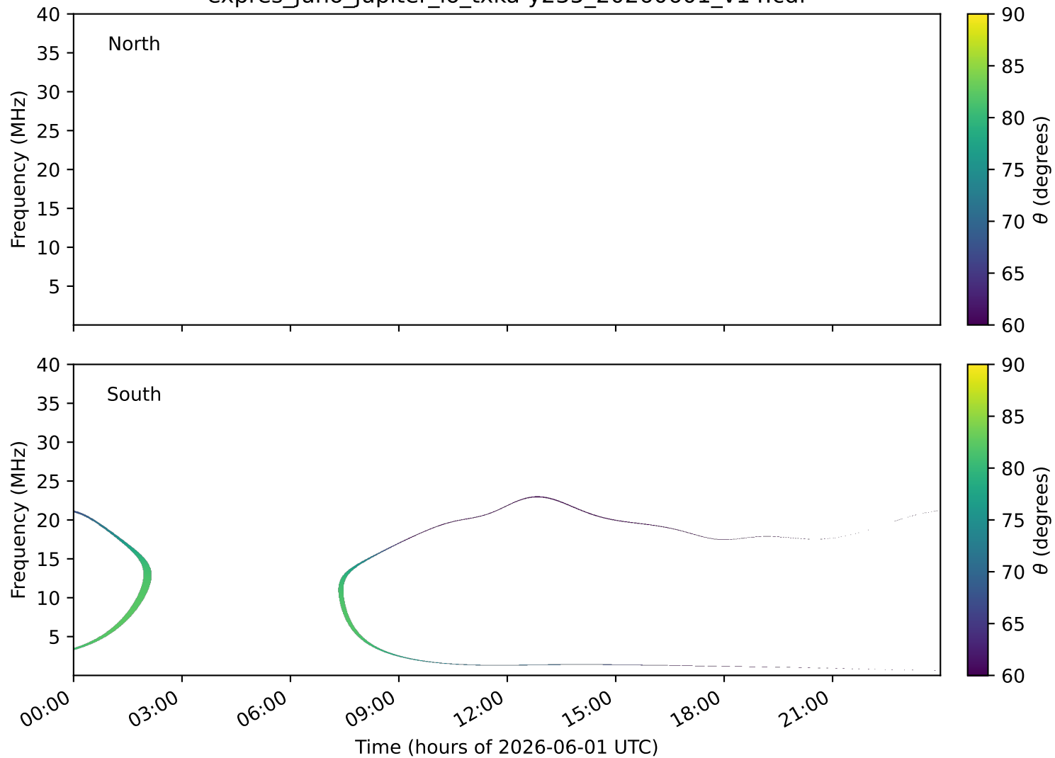
expres_juno_jupiter_io_txka-y235_20260601_v14.cdf
