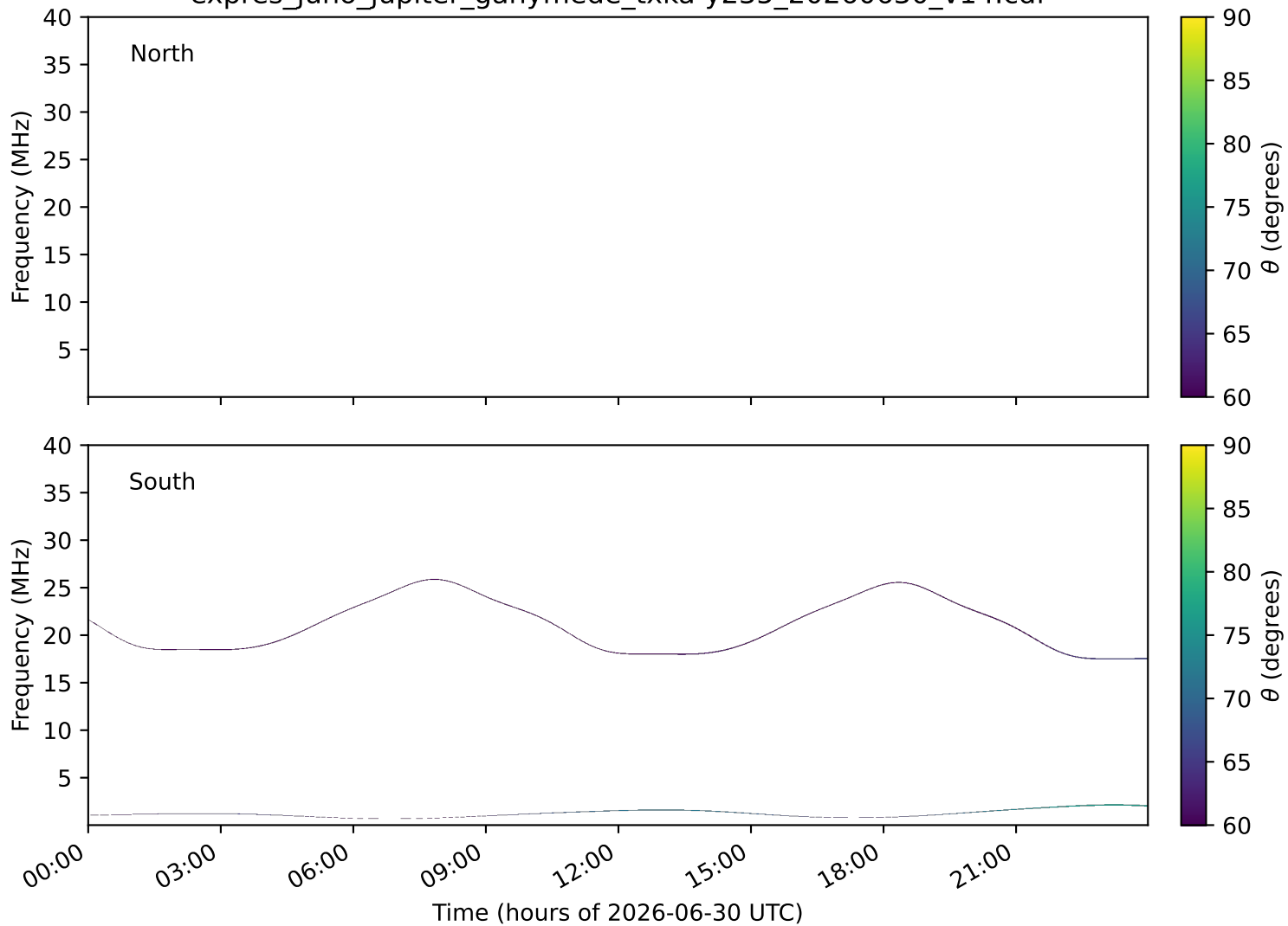
expres_juno_jupiter_ganymede_txka-y235_20260630_v14.cdf
