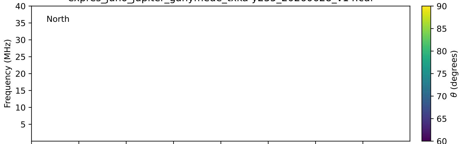
expres_juno_jupiter_ganymede_txka-y235_20260628_v14.cdf
