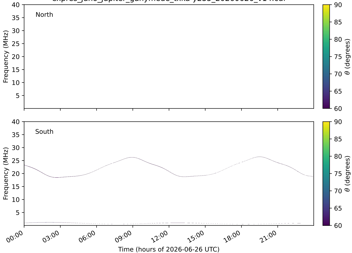
expres_juno_jupiter_ganymede_txka-y235_20260626_v14.cdf
