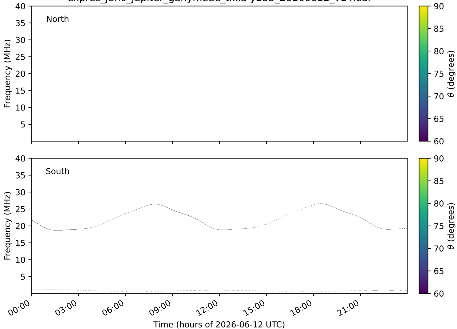
expres_juno_jupiter_ganymede_txka-y235_20260612_v14.cdf
