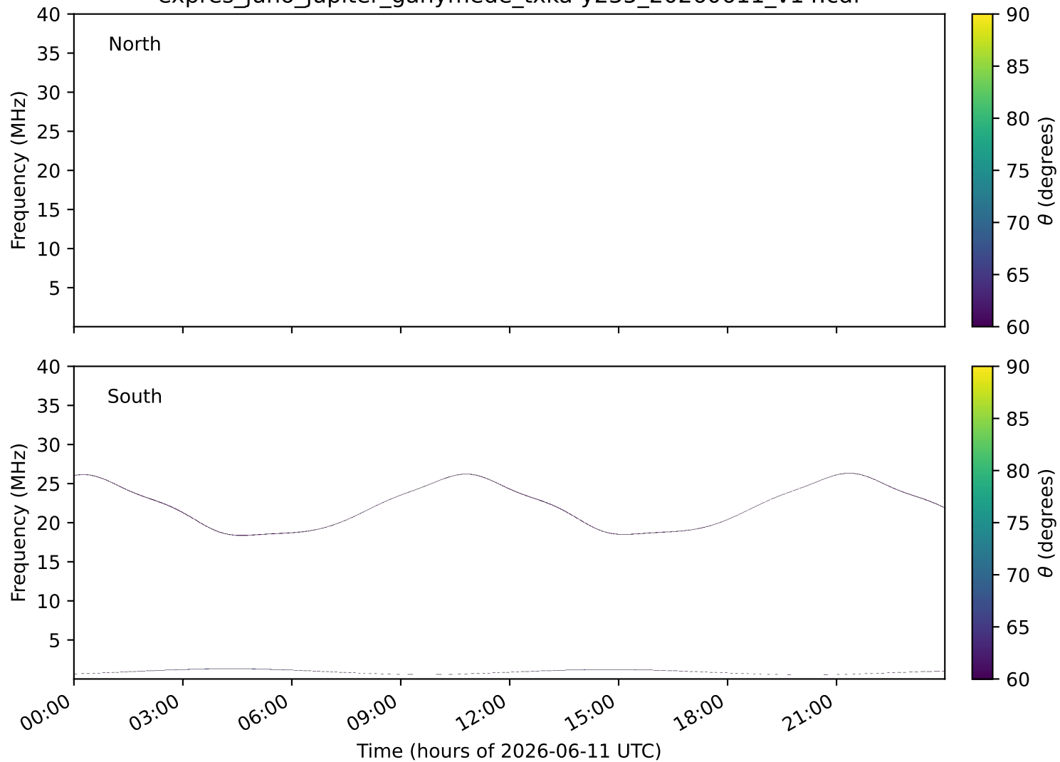
expres_juno_jupiter_ganymede_txka-y235_20260611_v14.cdf
