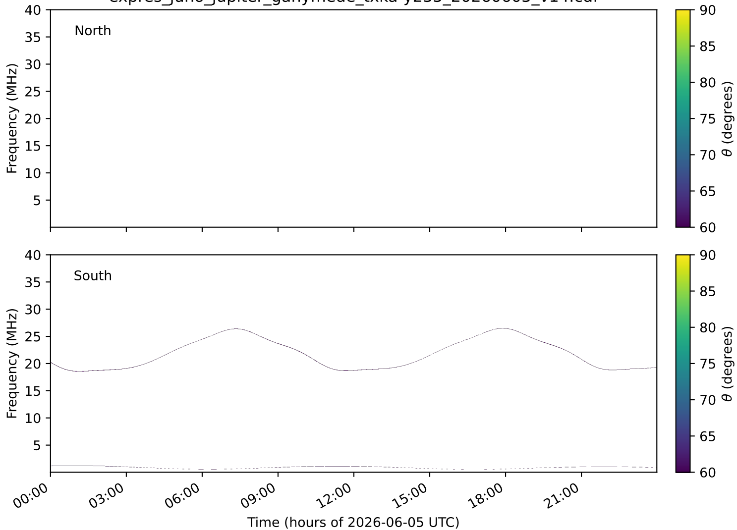
expres_juno_jupiter_ganymede_txka-y235_20260605_v14.cdf
