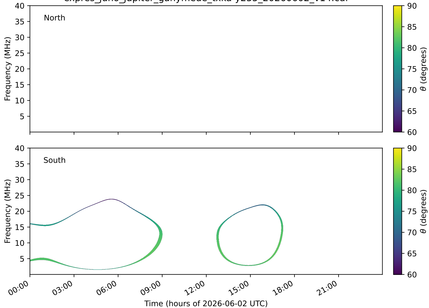
expres_juno_jupiter_ganymede_txka-y235_20260602_v14.cdf
