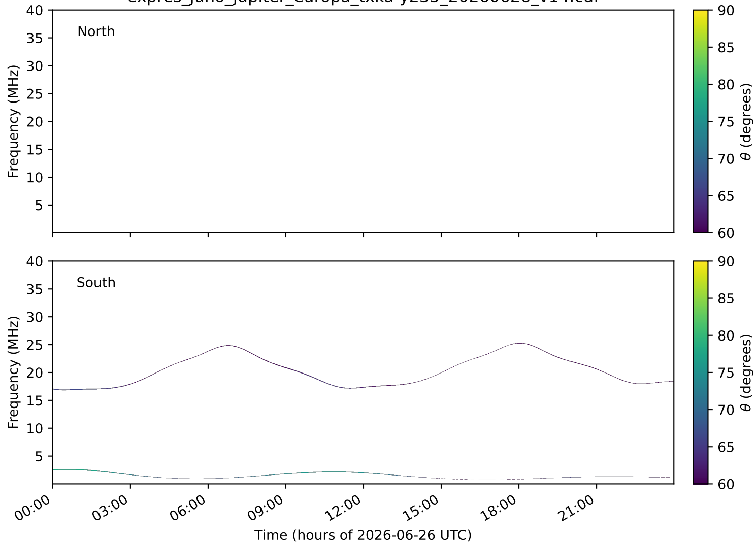
expres_juno_jupiter_europa_txka-y235_20260626_v14.cdf
