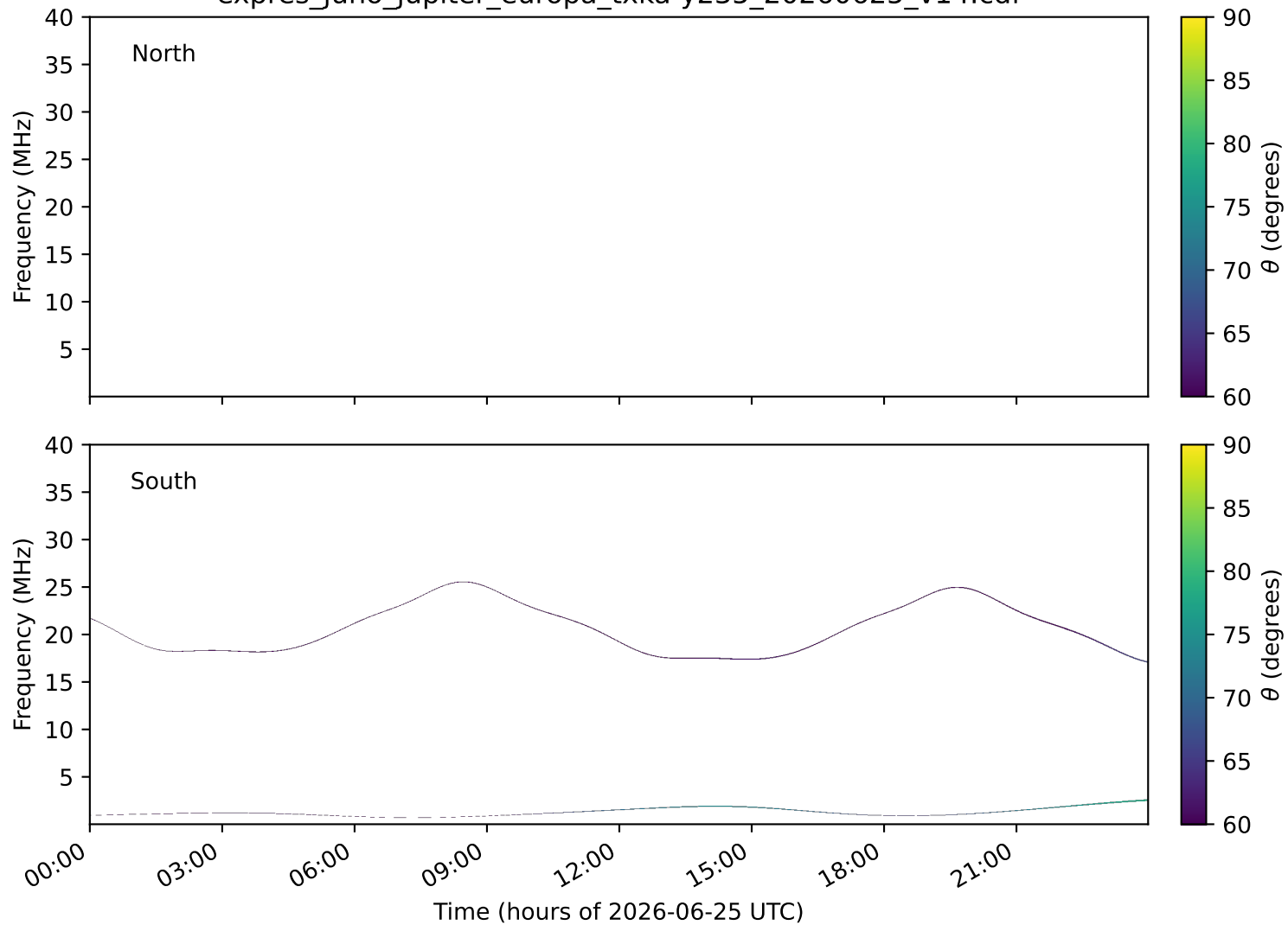
expres_juno_jupiter_europa_txka-y235_20260625_v14.cdf
