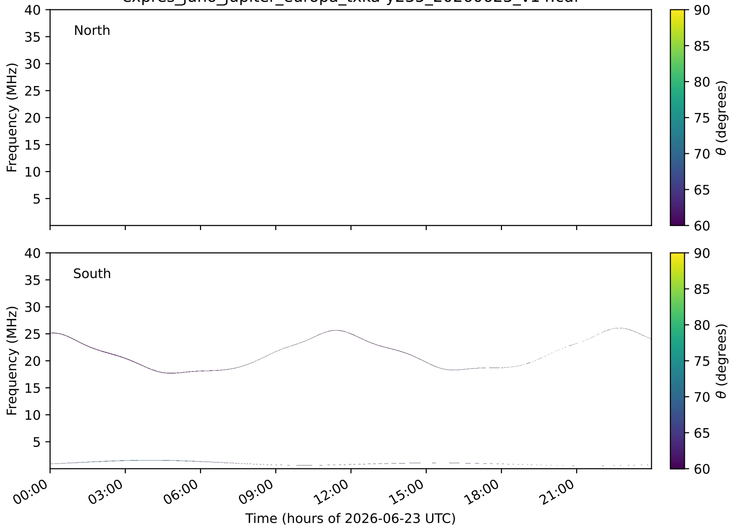
expres_juno_jupiter_europa_txka-y235_20260623_v14.cdf
