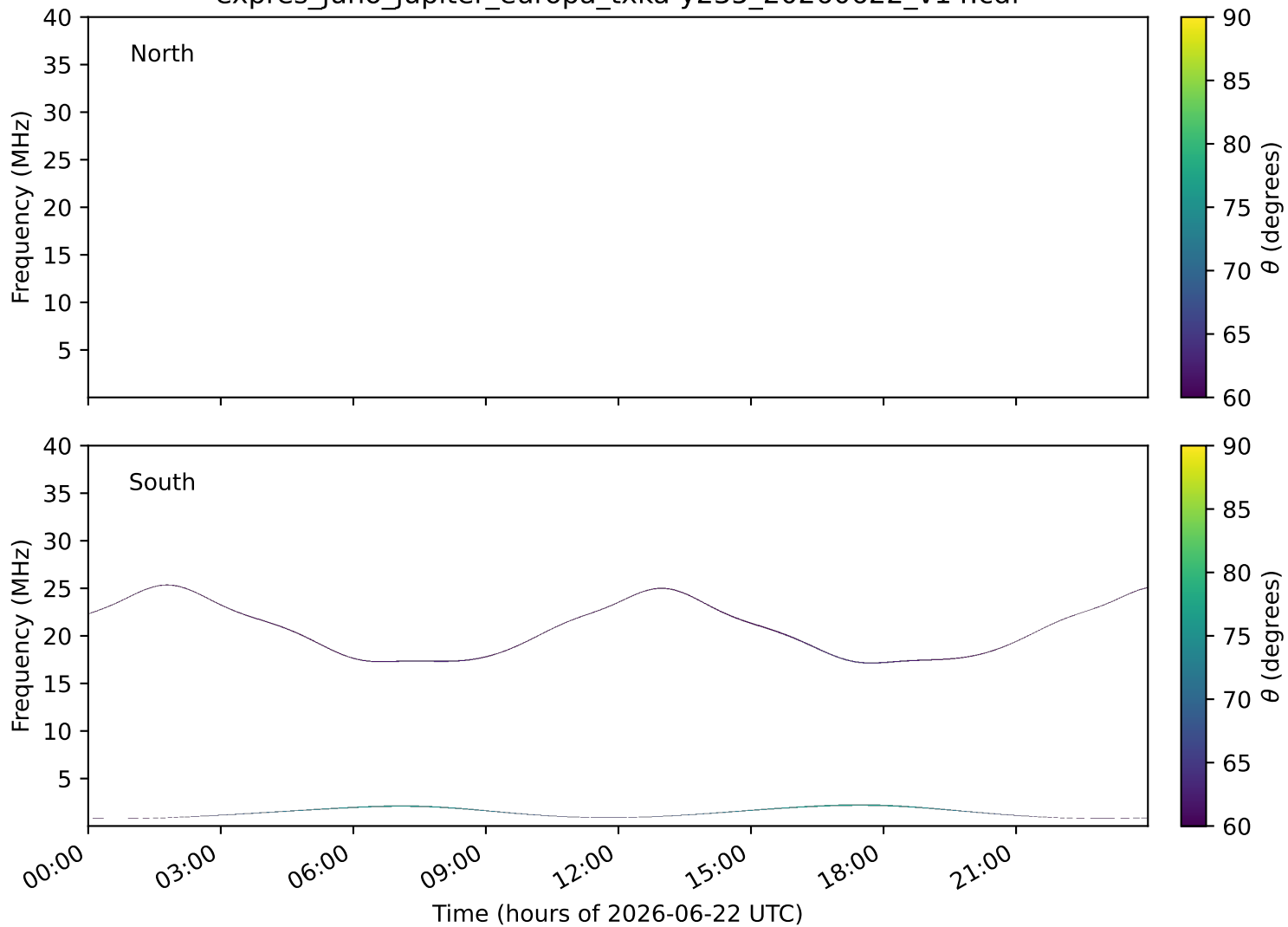
expres_juno_jupiter_europa_txka-y235_20260622_v14.cdf
