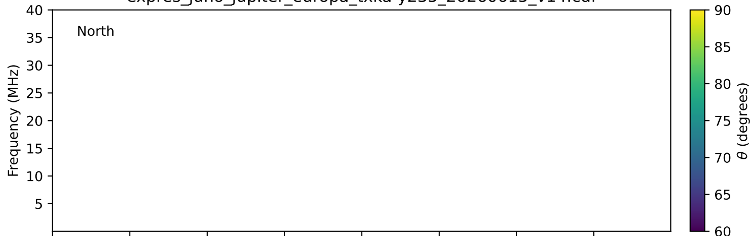
expres_juno_jupiter_europa_txka-y235_20260615_v14.cdf
