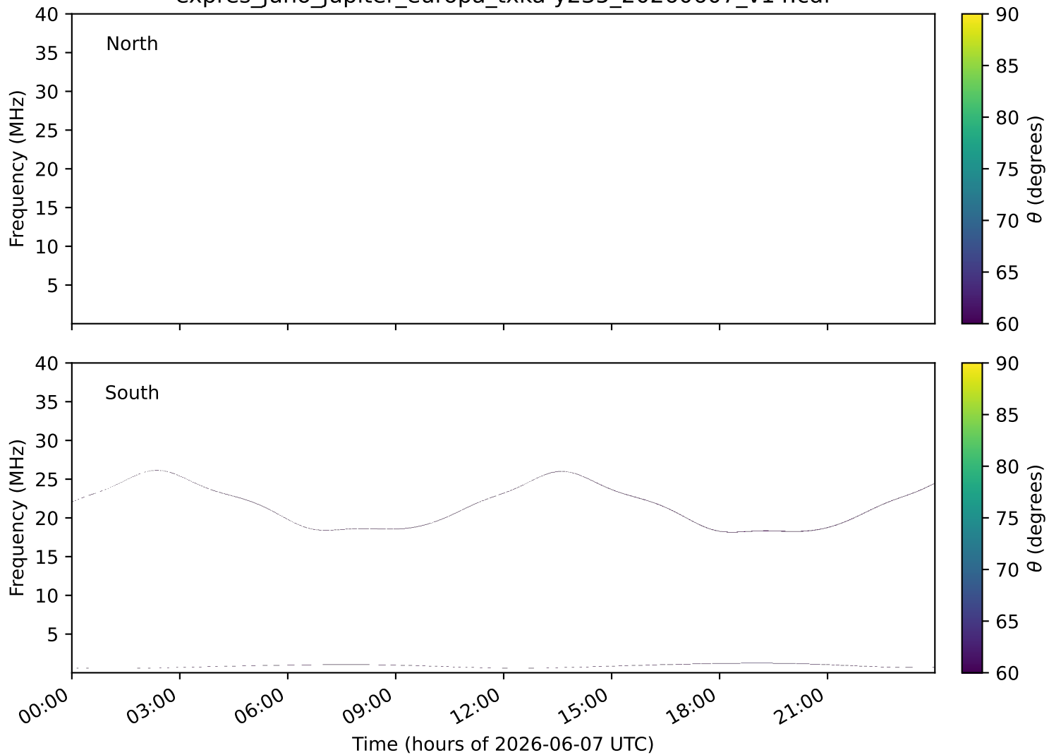
expres_juno_jupiter_europa_txka-y235_20260607_v14.cdf
