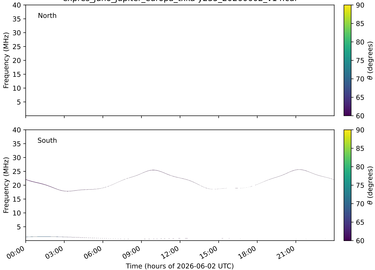
expres_juno_jupiter_europa_txka-y235_20260602_v14.cdf
