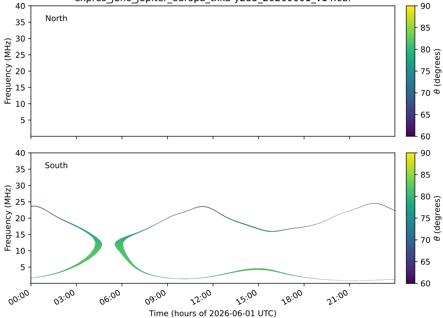
expres_juno_jupiter_europa_txka-y235_20260601_v14.cdf
