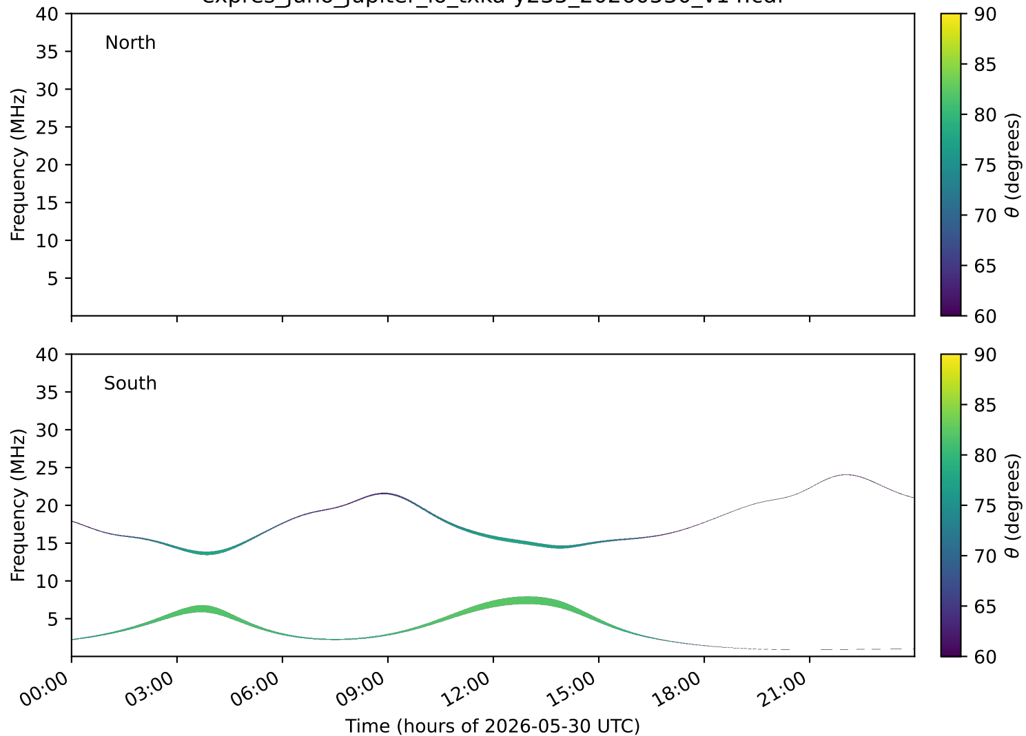
expres_juno_jupiter_io_txka-y235_20260530_v14.cdf
