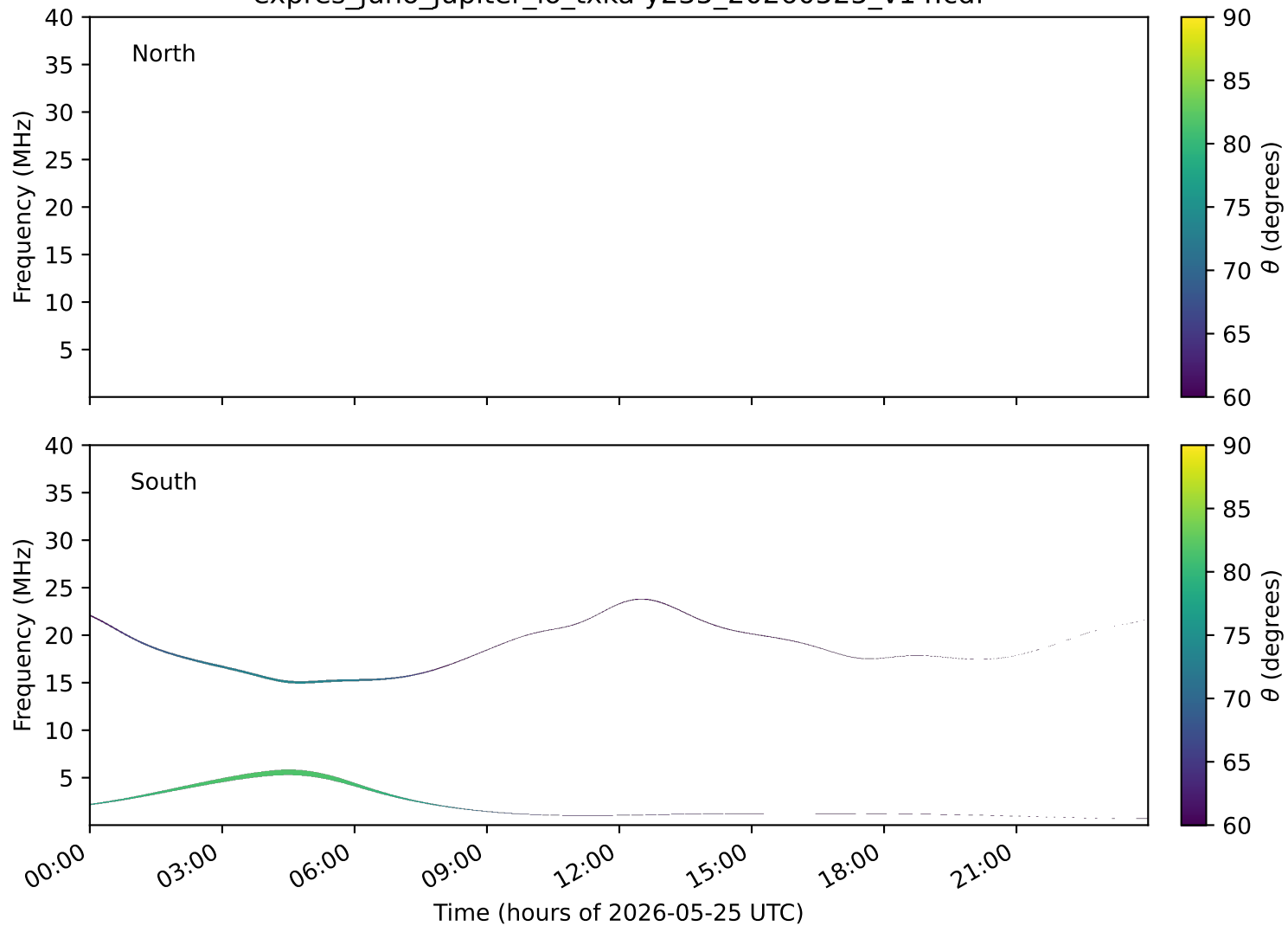
expres_juno_jupiter_io_txka-y235_20260525_v14.cdf
